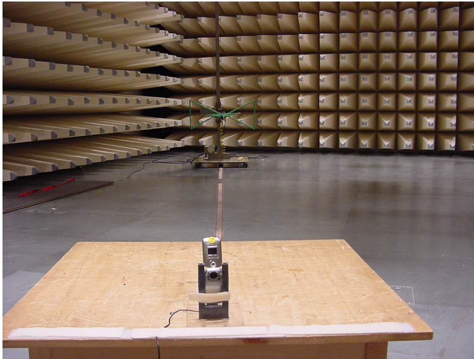
Photo 1: Radiated Emissions
