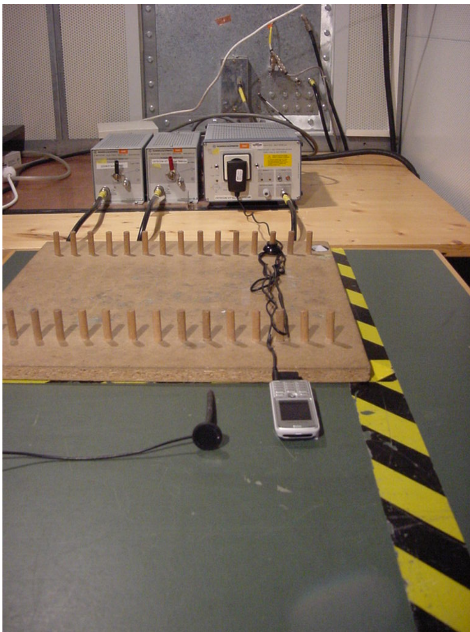
Photo 3 (Conducted Emissions):
