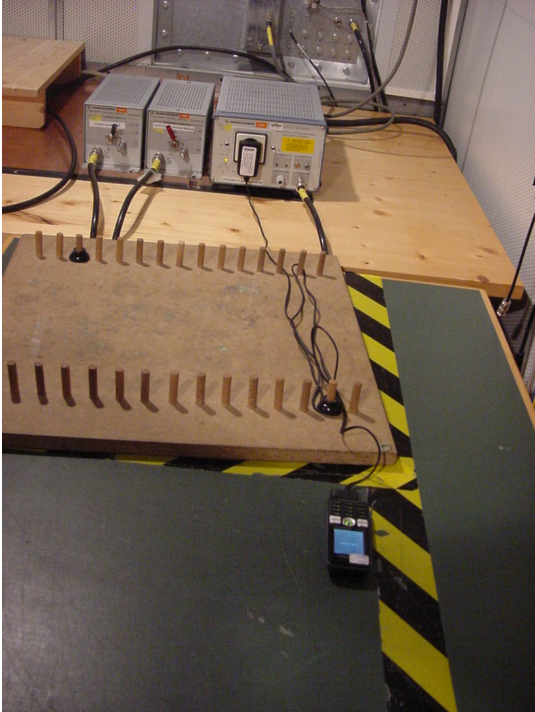
Photo 3: Conducted Emissions
