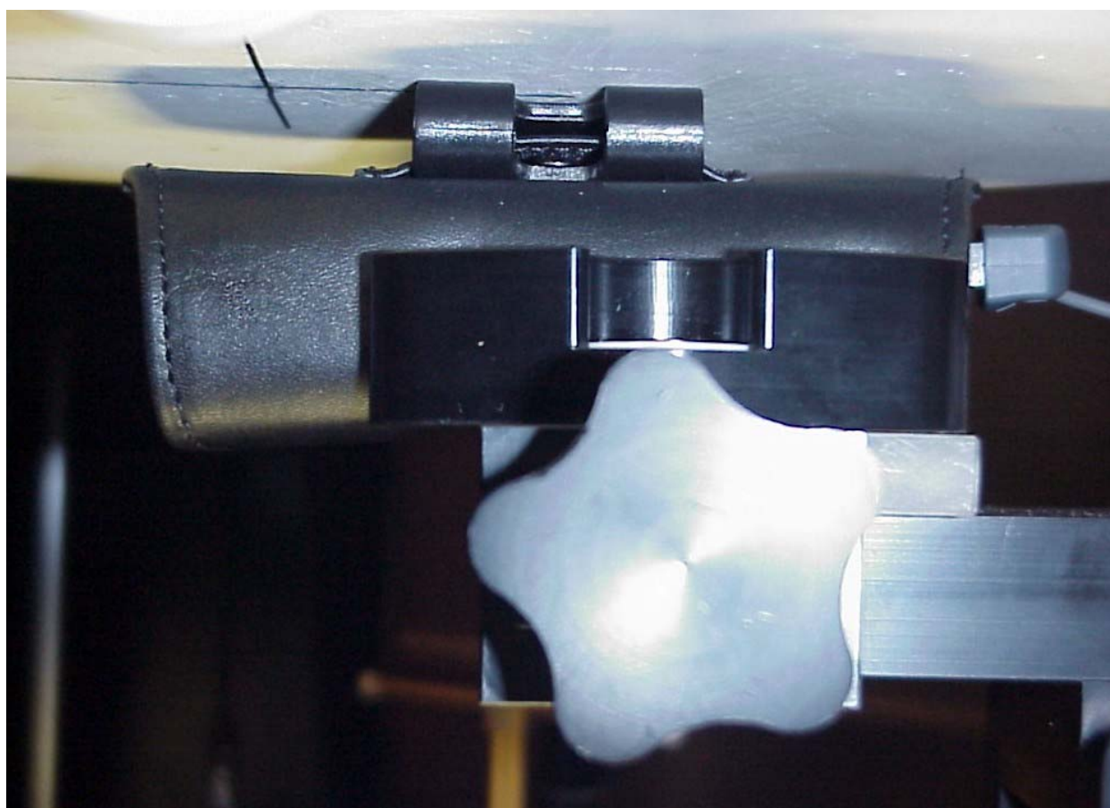
Position of device against flat phantom using carry accessory ICE-25 with hands free accessory RLF 501 25/04 (HPE-14).
