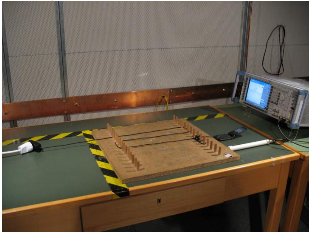
Photo 3 (Conducted Emissions):
