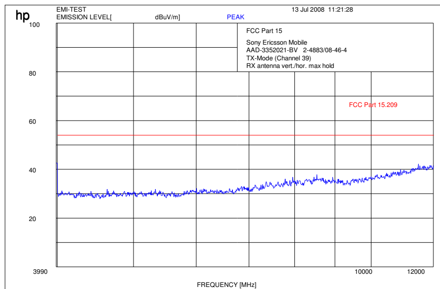
Plot 7: 4 - 12 GHz vertical/horizontal (middle channel)
