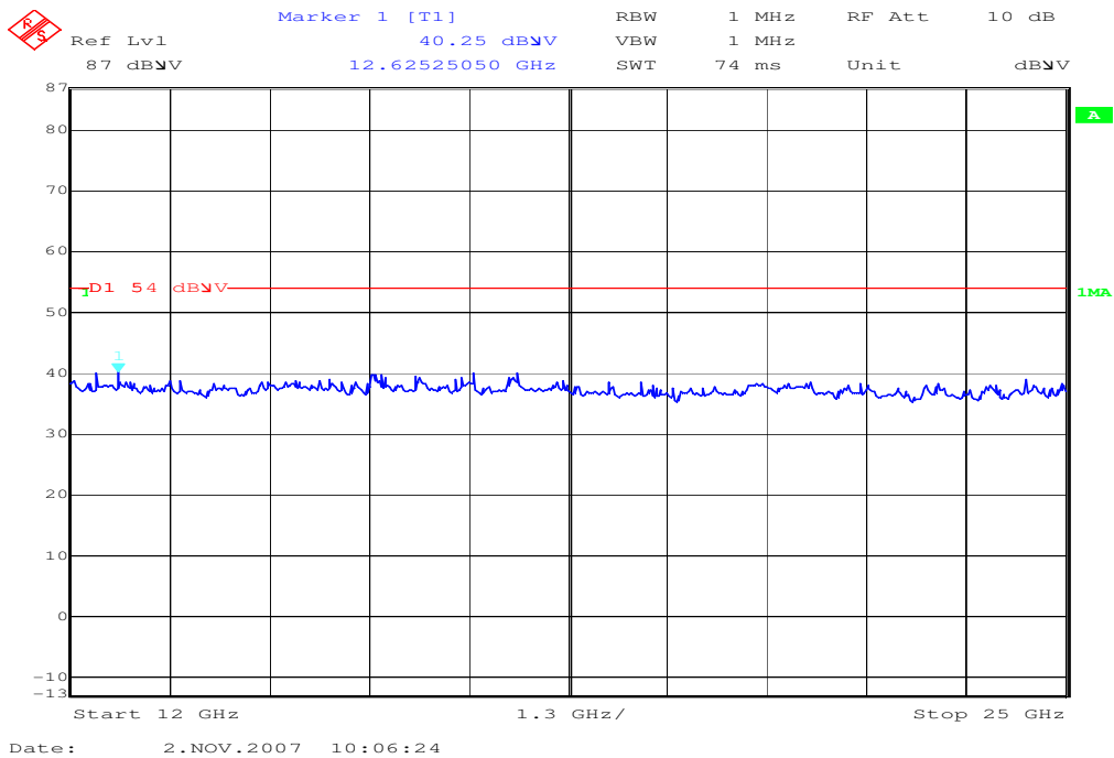
Plot 4: (Part 24) RX (12 GHz to 25 GHz)
