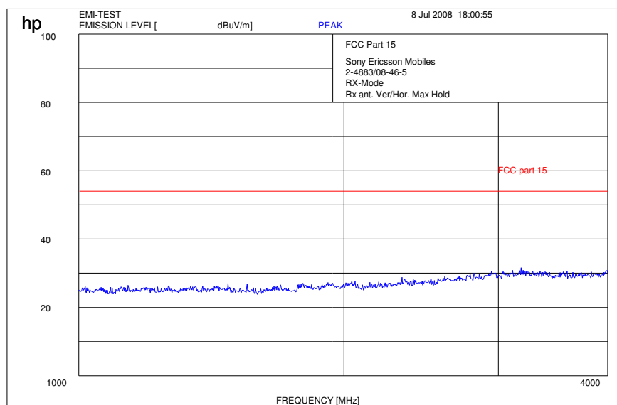
Plot 2: 1 - 4 GHz vertical / horizontal (receiver)
