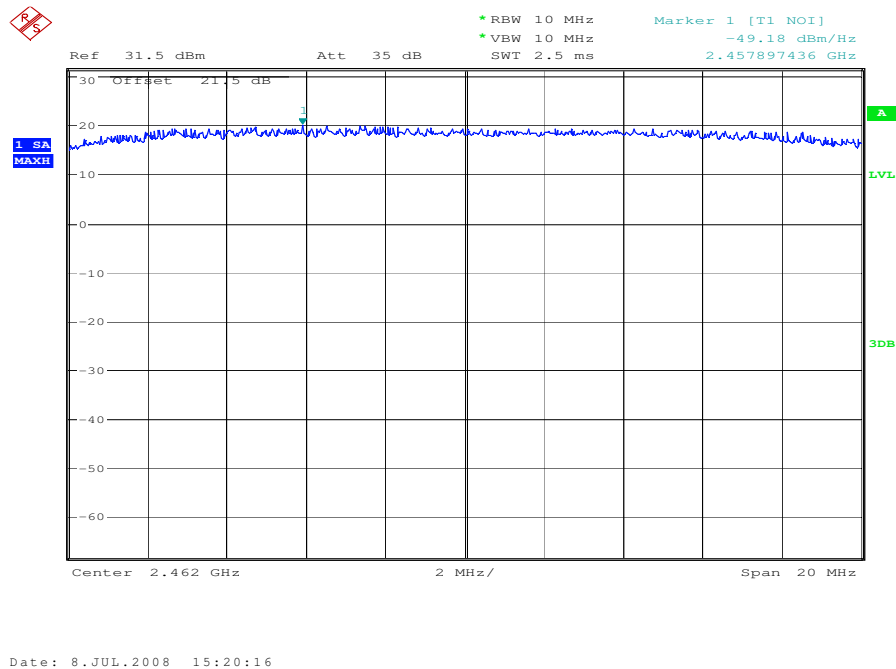
Plot 3: (result calculated by the Signal analyzer FSU from Rohde & Schwarz)
