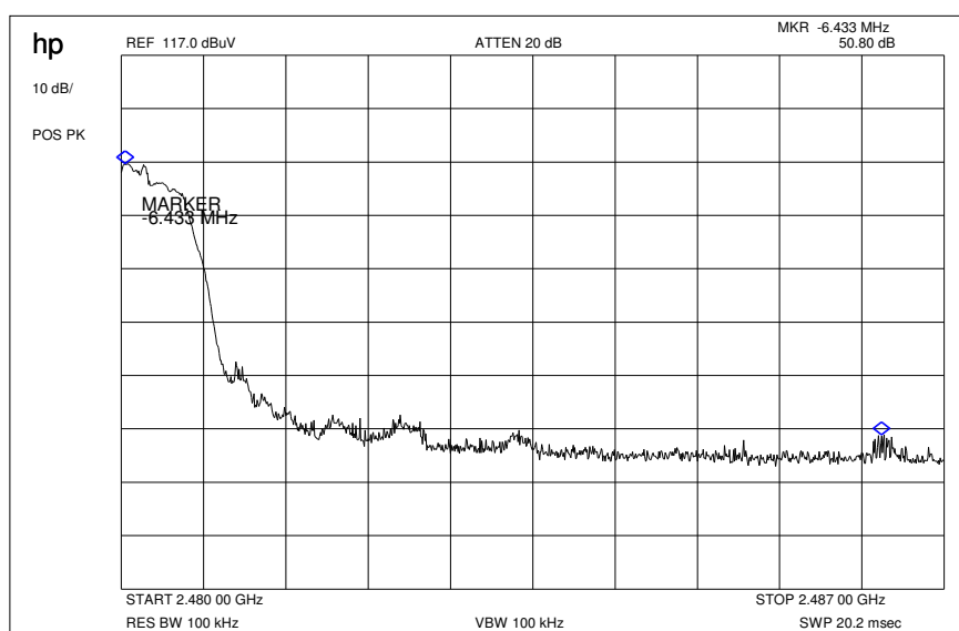
Plot 2: Marker-Delta Method (single carrier)
