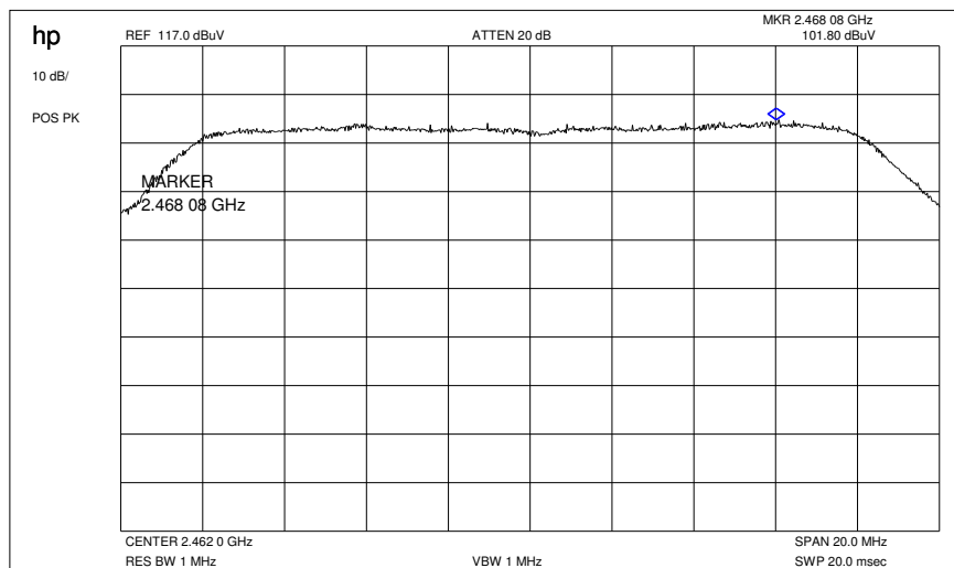
Plot 1: Max field strength in 3m distance (single frequency) peak
