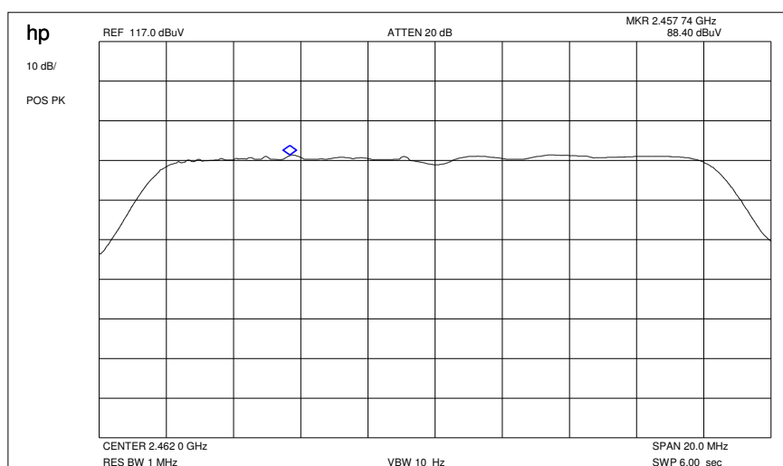
Plot 2 : Max field strength in 3m distance (single frequency) average
