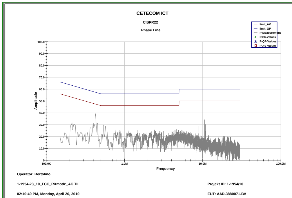
Plot 2: RX / Idle mode; phase line
