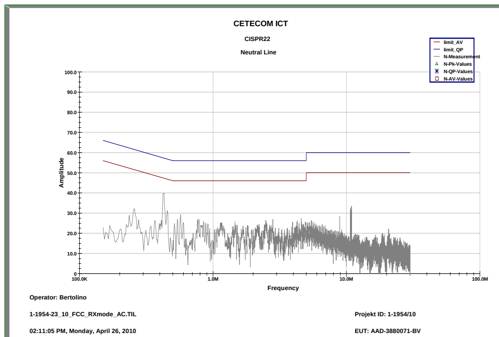
Plot 1: RX / Idle mode; neutral line
