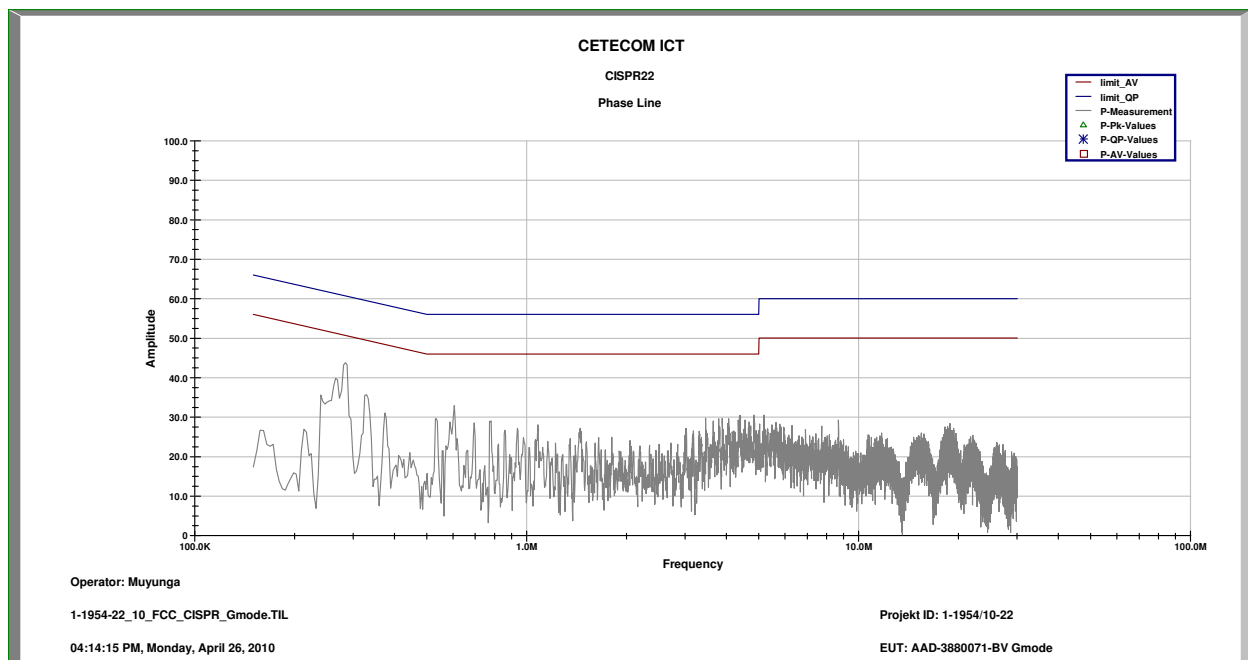
Plot 2: CISPR 22
