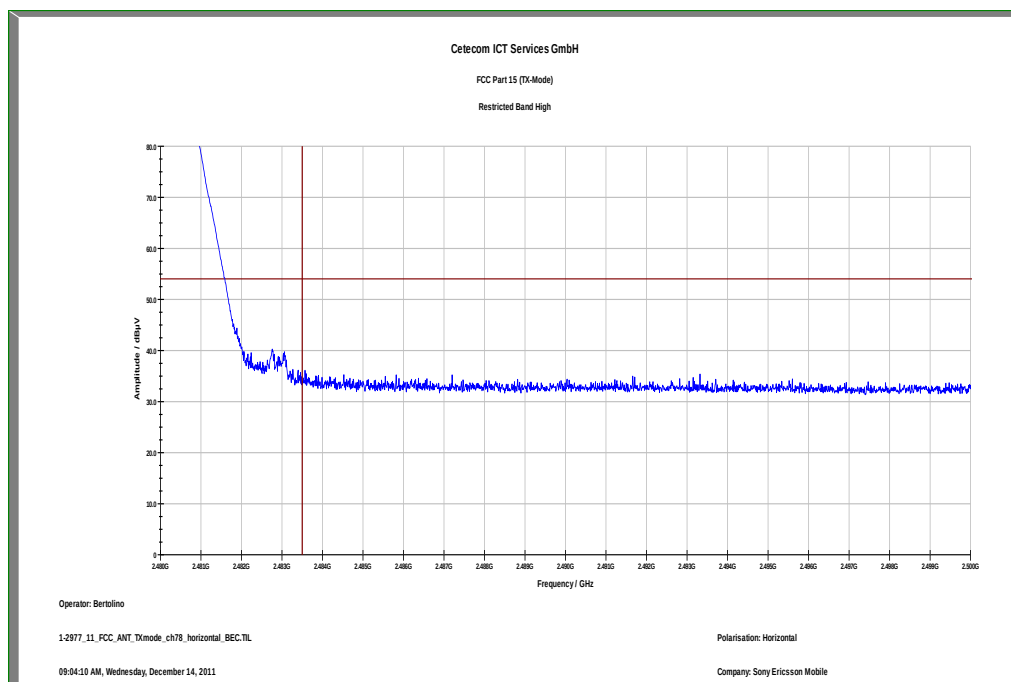
Plot 4: upper band edge, horizontal polarization
