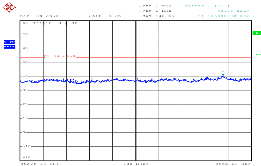
Plot 15: Highest channel, 18 GHz to 25 GHz, vertical & horizontal polarization
