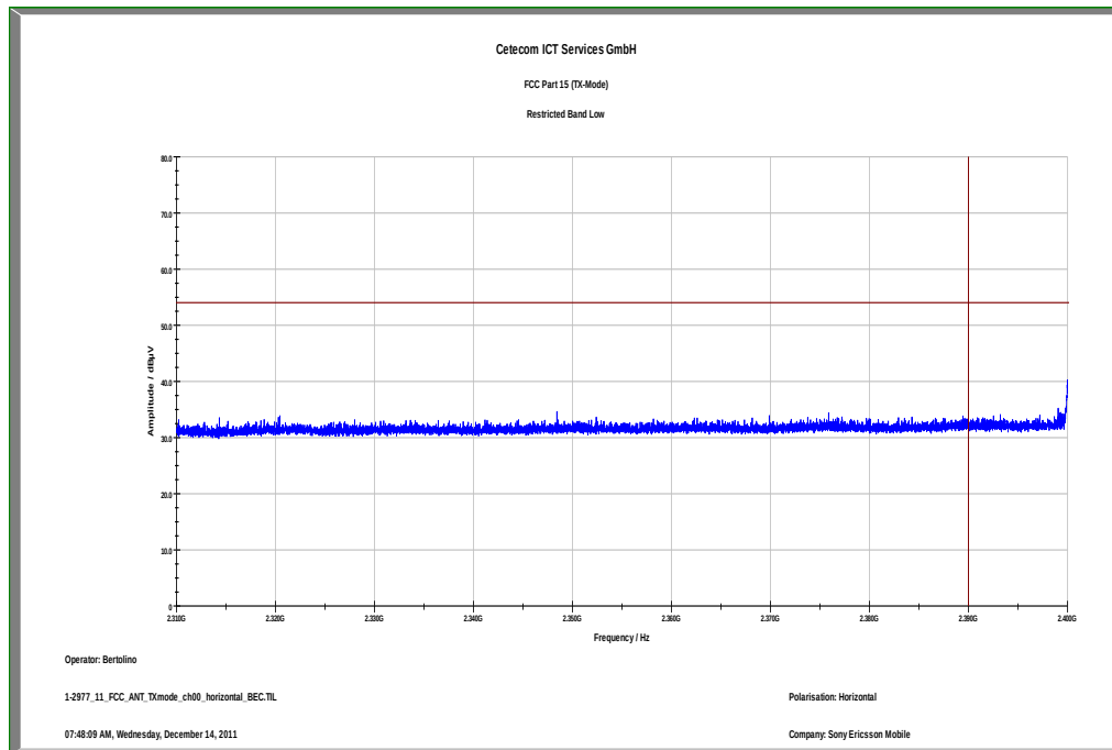
Plot 3: lower band edge, horizontal polarization
