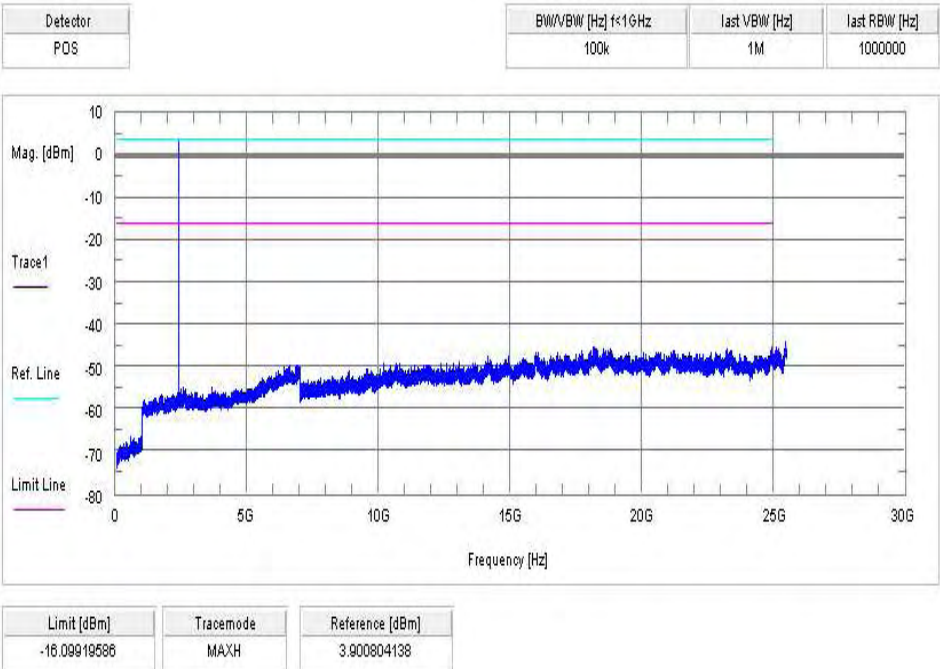
Plot 4: lowest channel – 2402 MHz, Pi / DQPSK modulation
