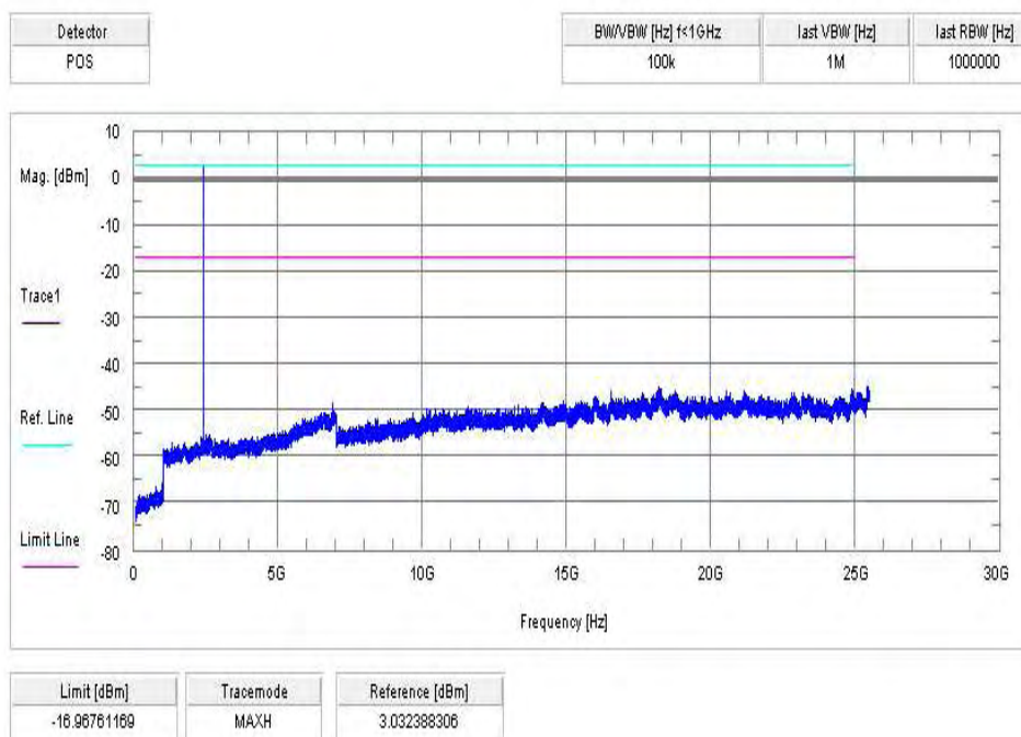
Plot 7: lowest channel – 2402 MHz, 8 DPSK modulation
