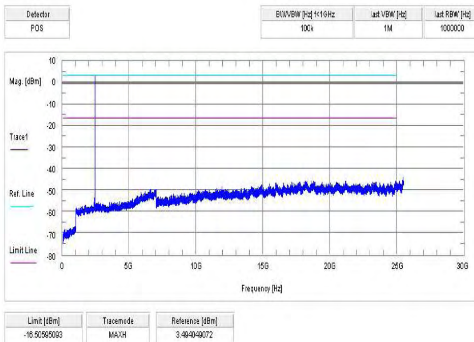
Plot 8: middle channel – 2441 MHz, 8 DPSK modulation
