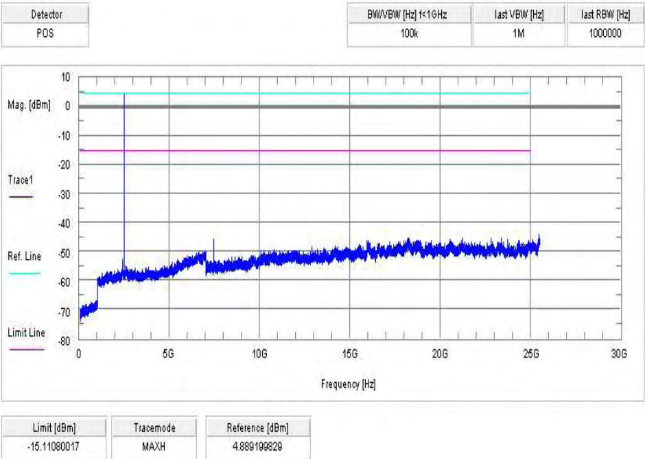
Plot 6: highest channel – 2480 MHz, Pi / DQPSK modulation
