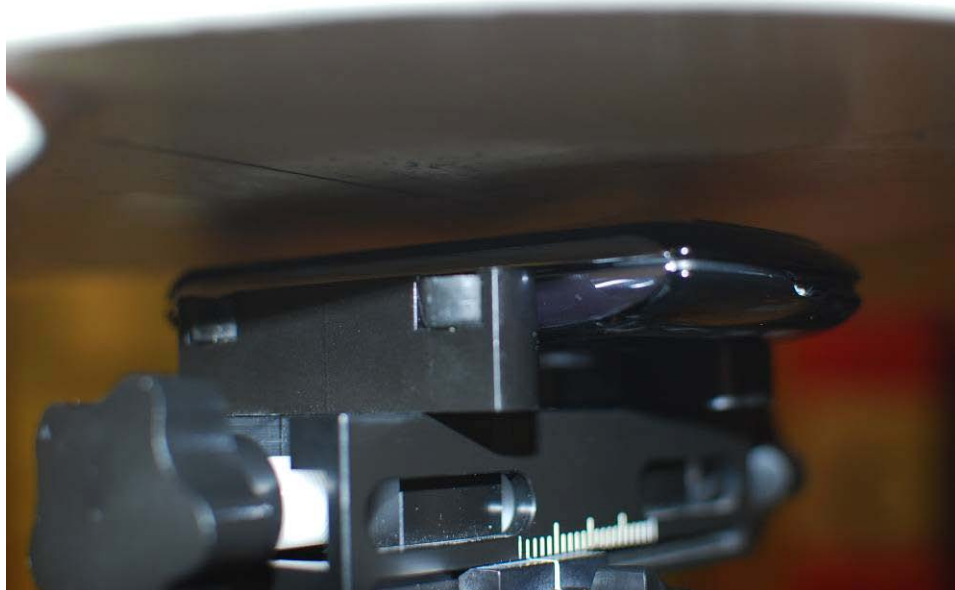
Figure 21-6 SAR Test Setup Photo – Front at 1.0 cm
