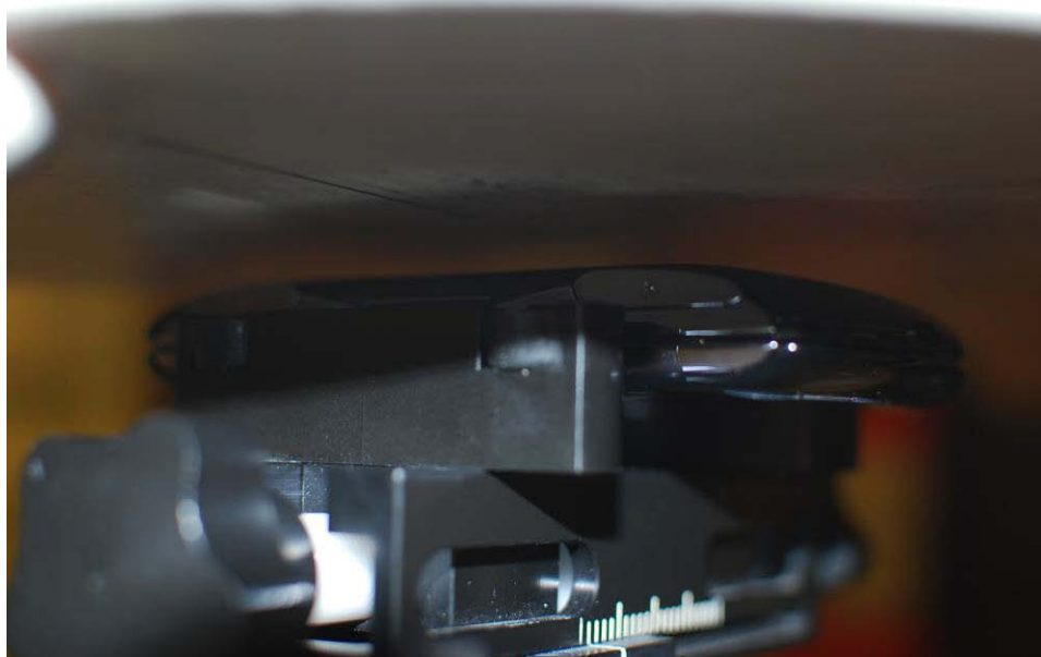
Figure 21-5 SAR Test Setup Photo – Back at 1.0 cm
