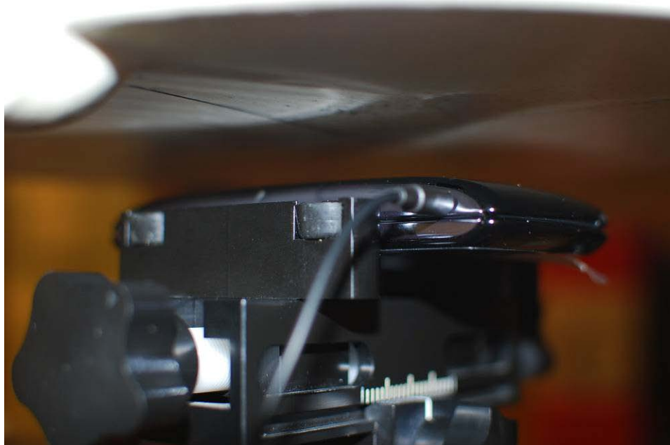
Figure 21-11 SAR Test Setup Photo – Back at 1.5 cm
