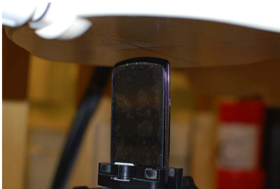
Figure 21-8 SAR Test Setup Photo – Bottom at 1.0 cm
