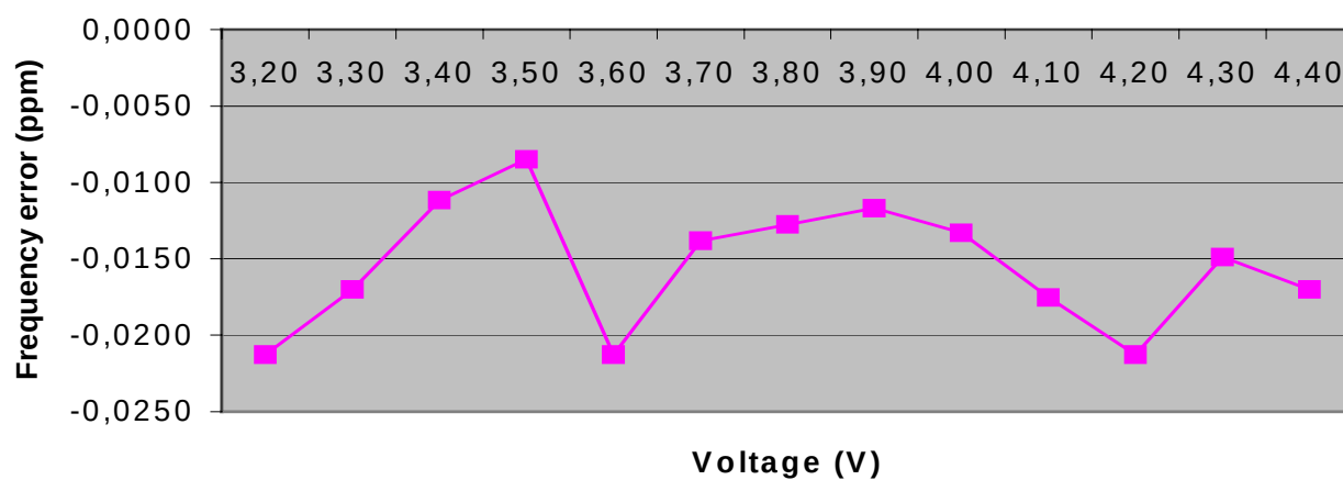
Frequency Error vs. Voltage
