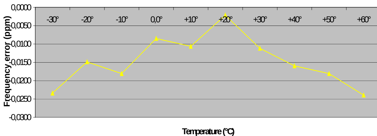
FREQUENCY ERROR VERSUS TEMPERATURE
