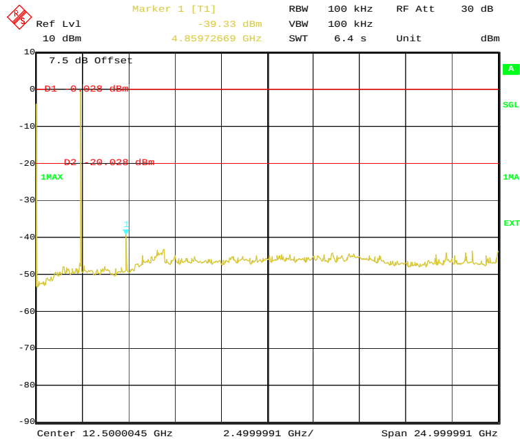
Plot 2 of 3: middle channel
