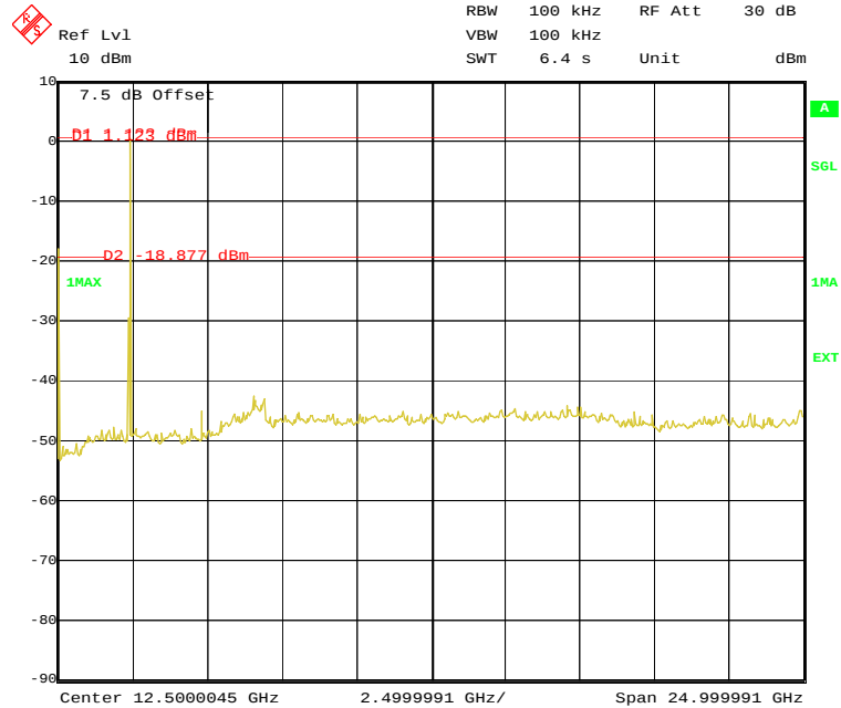
Plot 1 of 3: lowest channel
