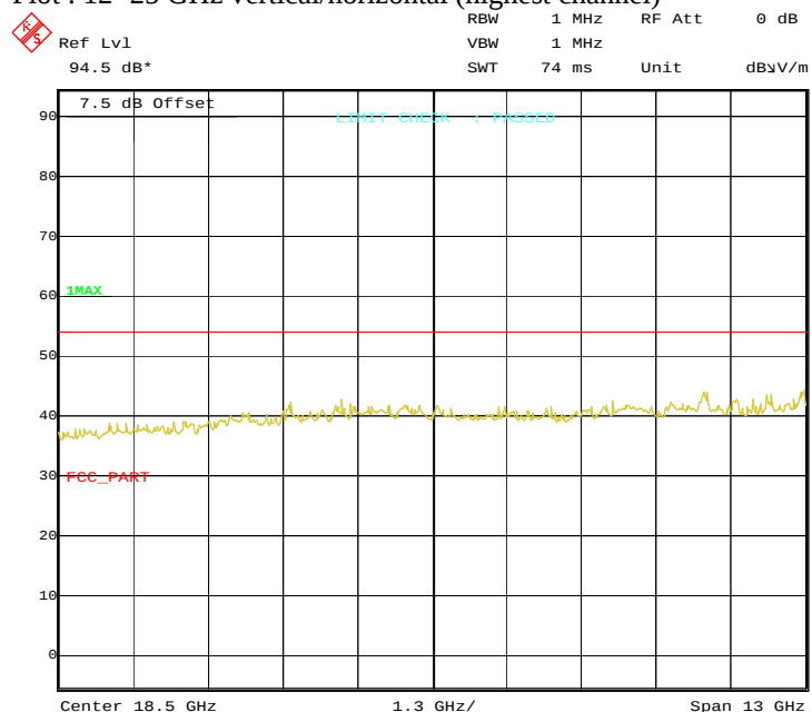
Plot : 12- 25 GHz vertical/horizontal (highest channel)
