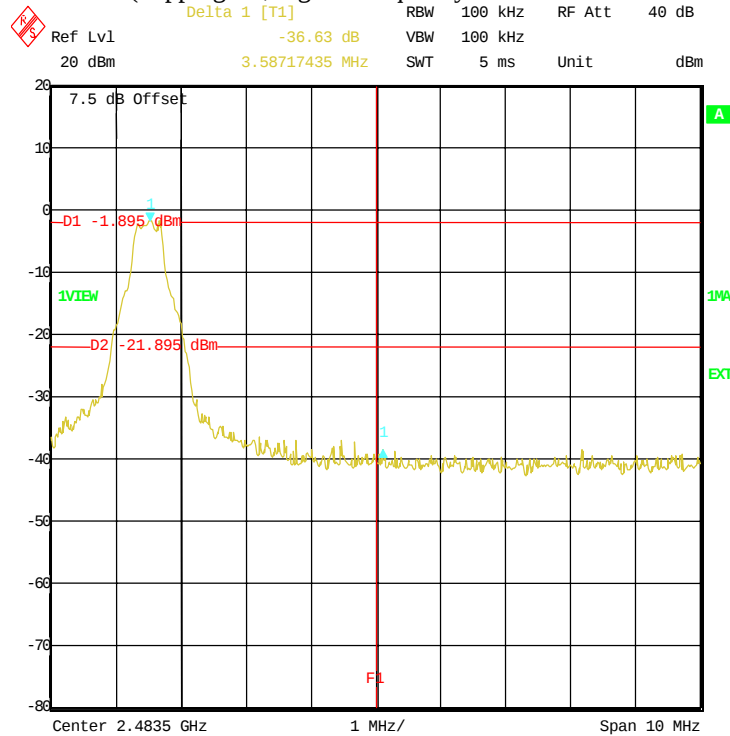
Plot 3 of 4 (hopping off, highest frequency)
