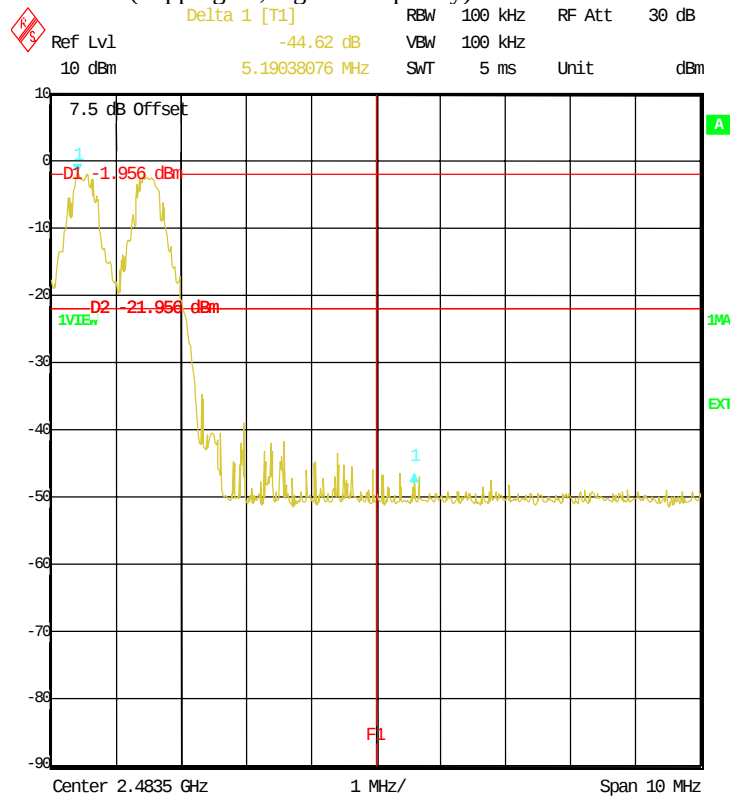
Plot 4 of 4 (hopping on, highest frequency):
