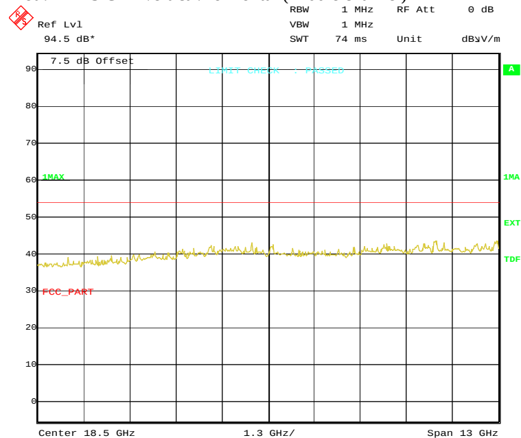
Plot : 12- 25 GHz vertical/horizontal (middle channel)
