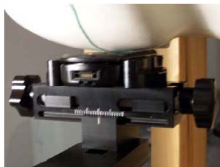
Device position against the head: Cheek (touch) phone position (phone in close state)
