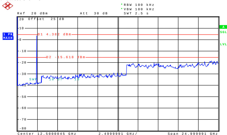
Plot 1 of 3: lowest channel
