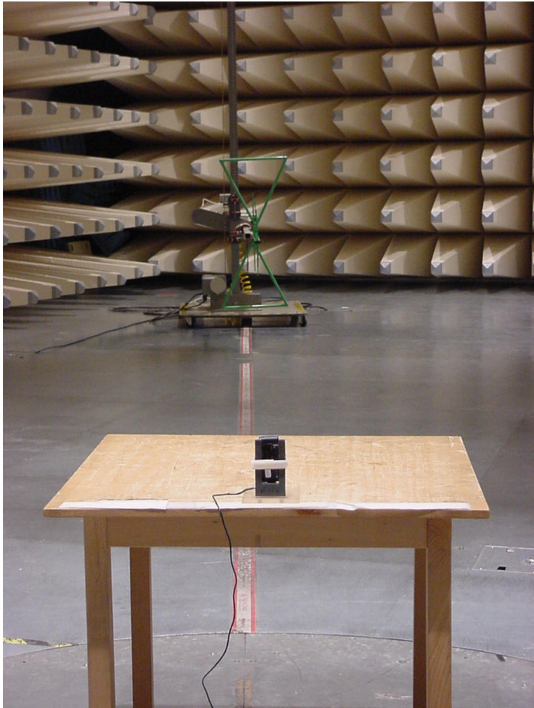
Photo 1 (Radiated Emissions):
