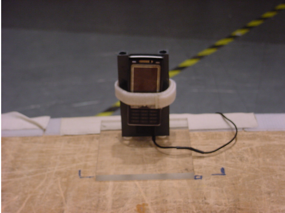
Photo 3 (Radiated Emissions):
