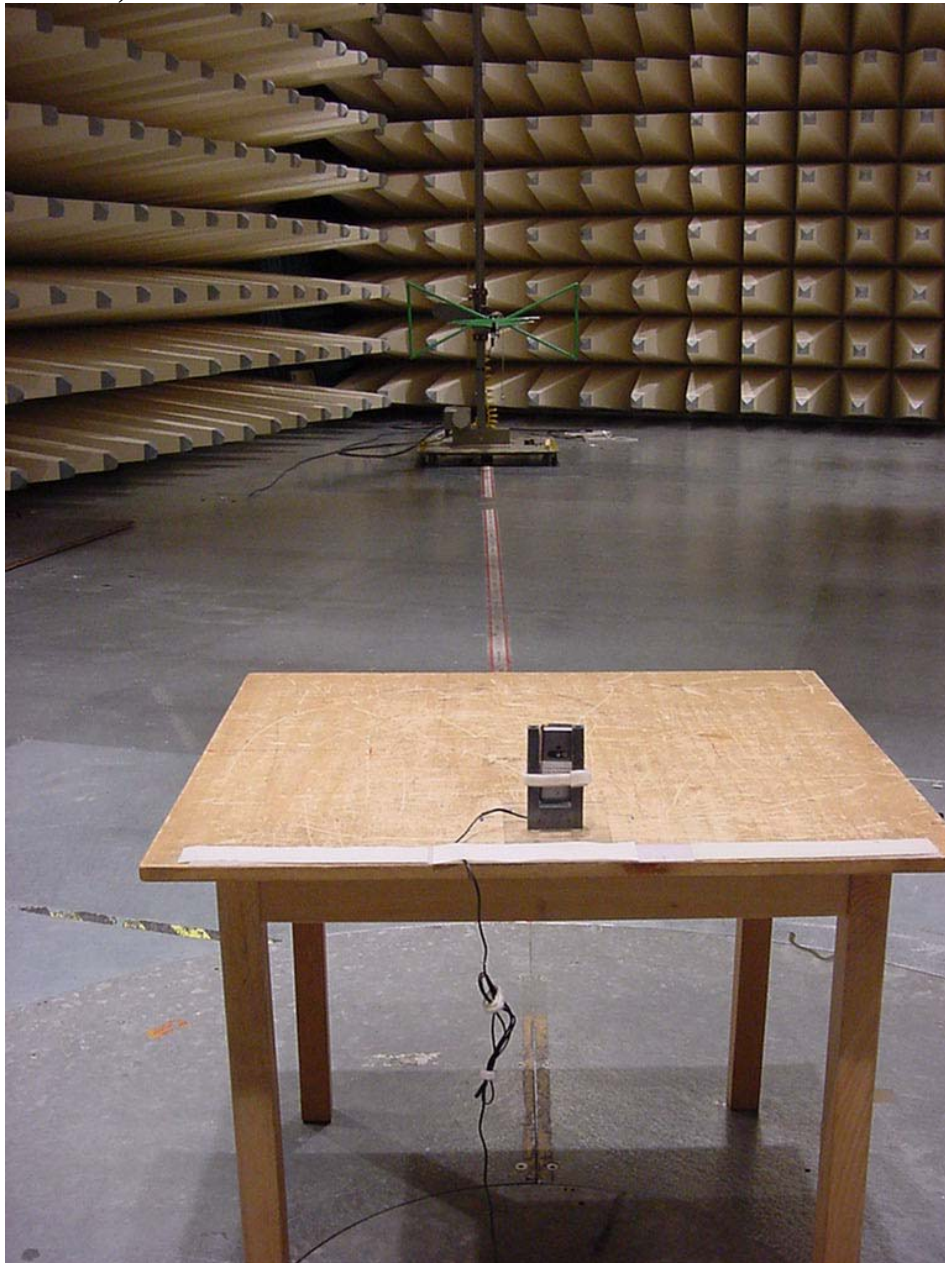
Photo 1 (Radiated Emissions):
