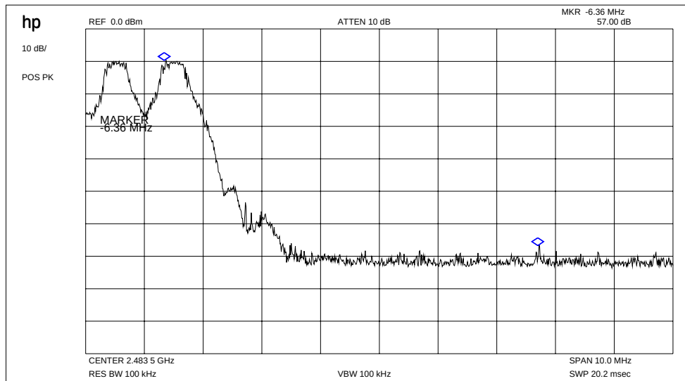
Plot 3: Marker-Delta Method (single carrier, channel 78)
