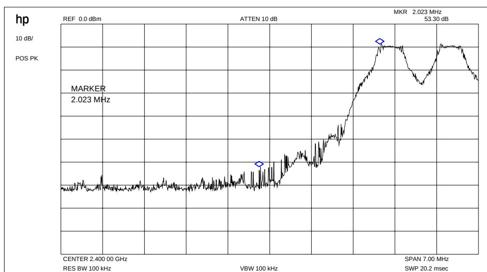
Plot 4: Marker-Delta Method (single carrier, channel 00)
