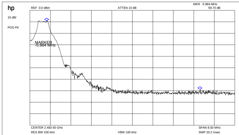
Plot 3: Marker-Delta Method (single carrier, channel 78)
