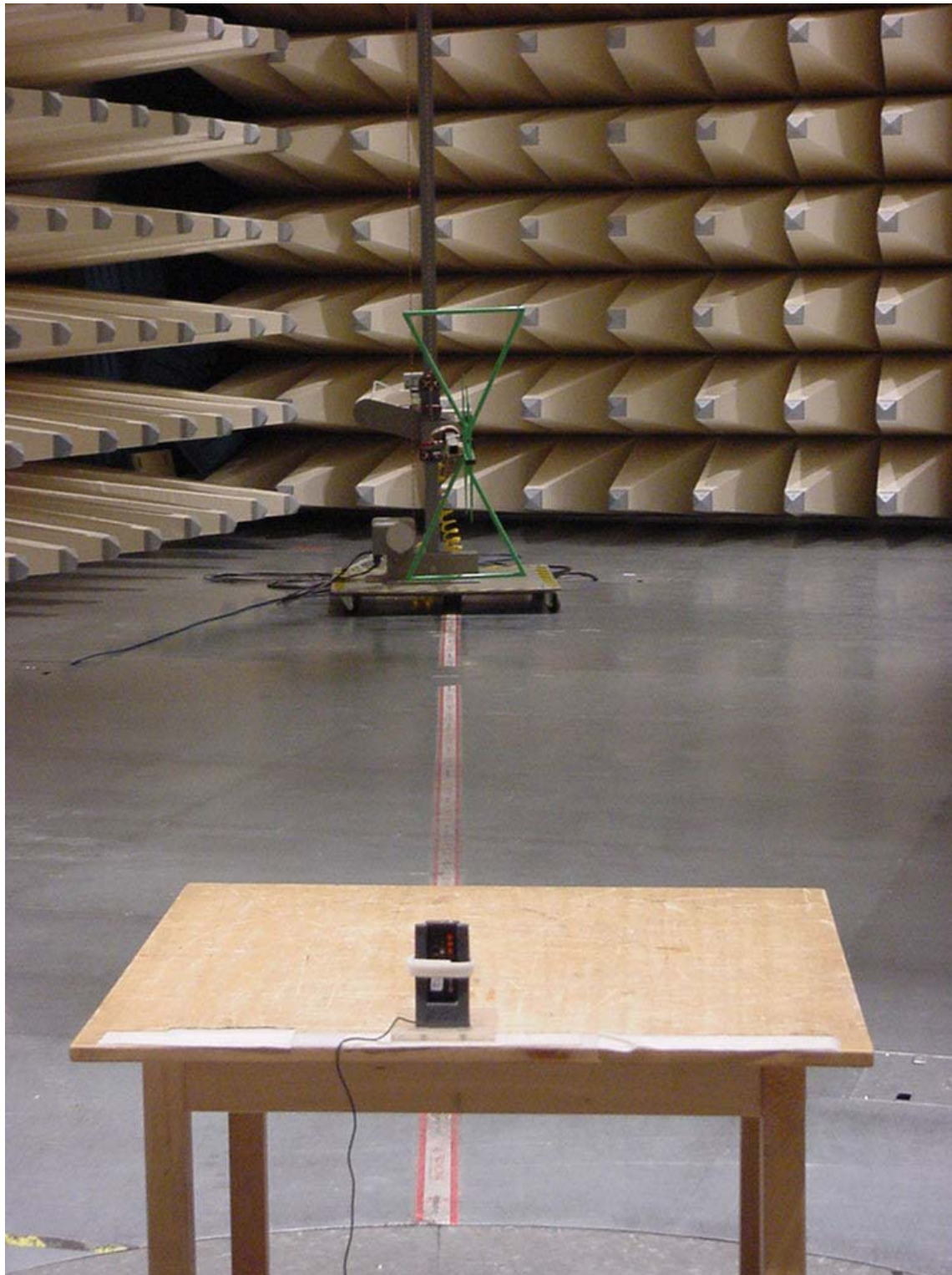
Photo 2 (Radiated Emissions):
