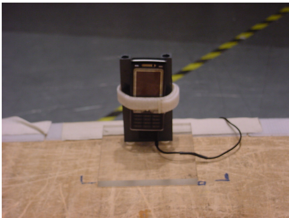
Photo 2 (Radiated Emissions):
