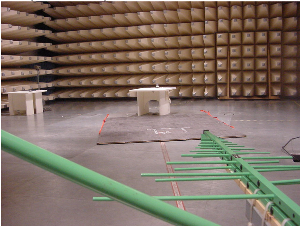
Photo 4 (Radiated Emissions):
