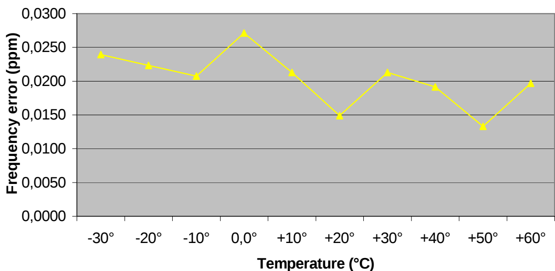
FREQUENCY ERROR VERSUS TEMPERATURE
