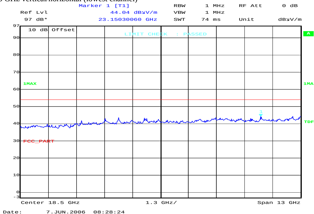
Plot : 12- 25 GHz vertical/horizontal (lowest channel)
