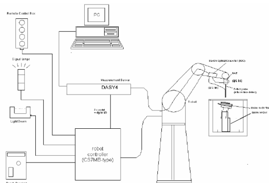
Figure 5-9 SPEAG Robotic System Diagram
