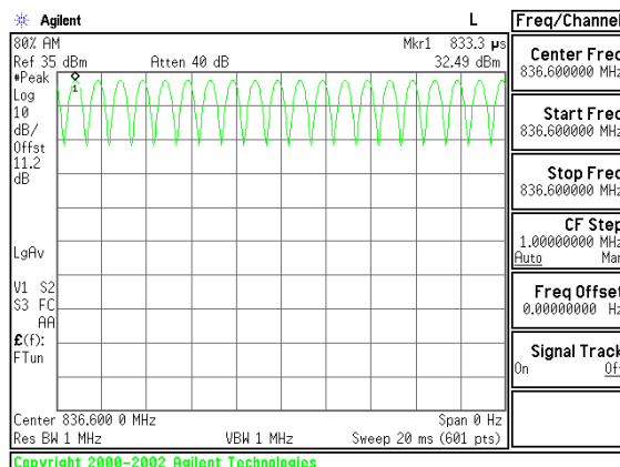
Figure 8-3 GSM850 80% AM Signal
