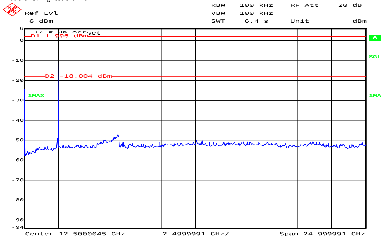
Plot 3 of 3: highest channel
