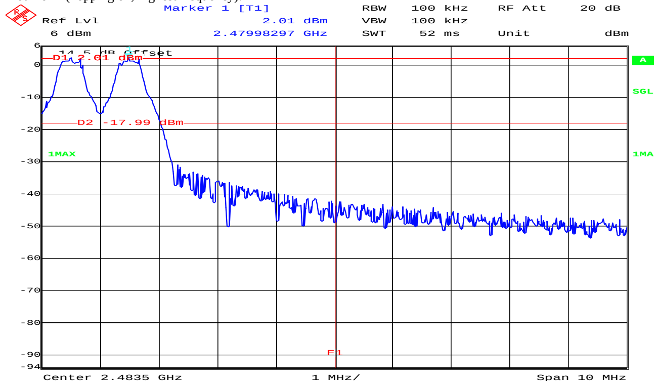
Plot 4 of 4 (hopping on, highest frequency):
