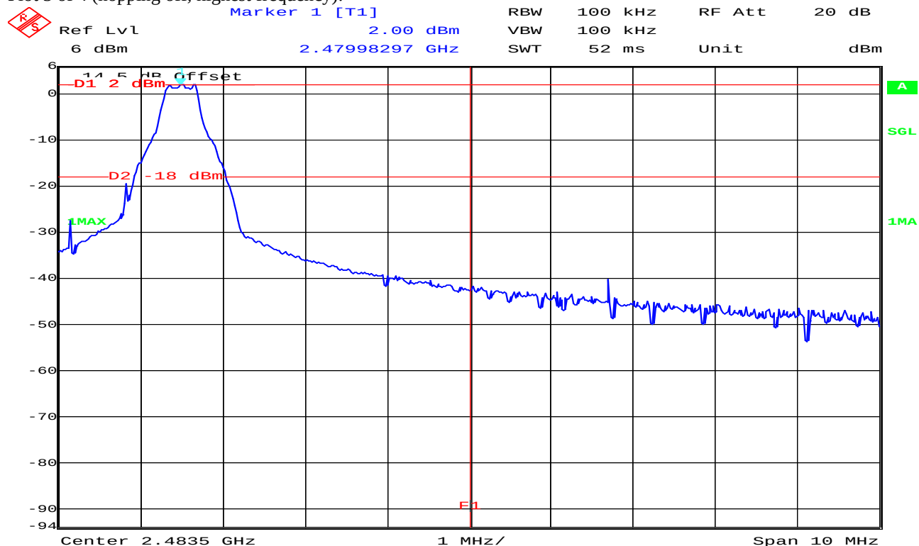
Plot 3 of 4 (hopping off, highest frequency):
