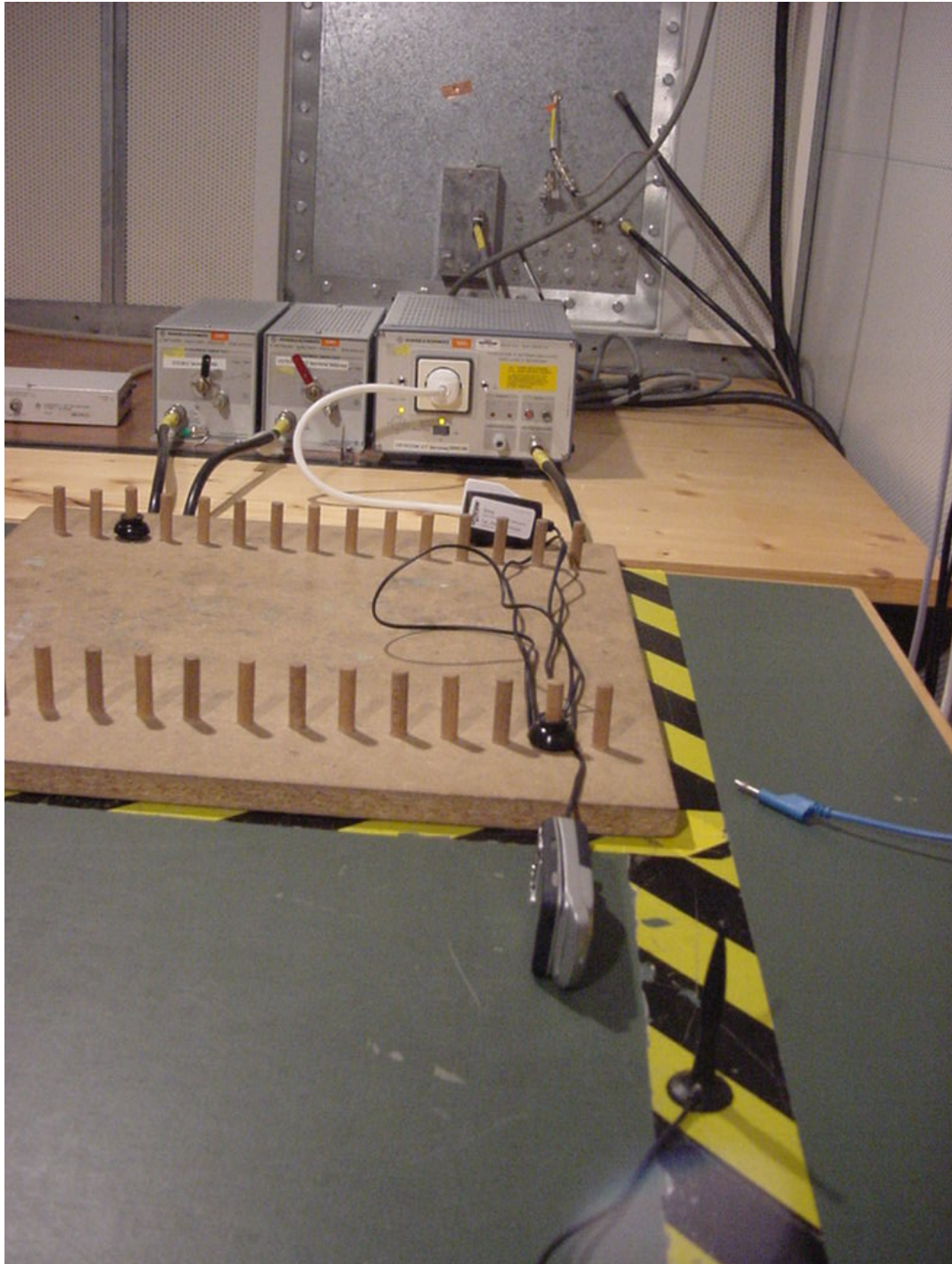
Photo 3: Conducted Emissions
