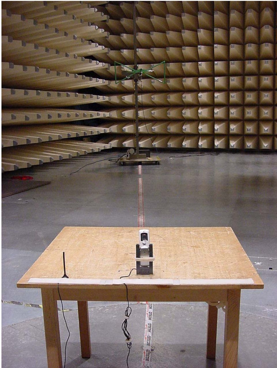
Photo 1: Radiated Emissions
