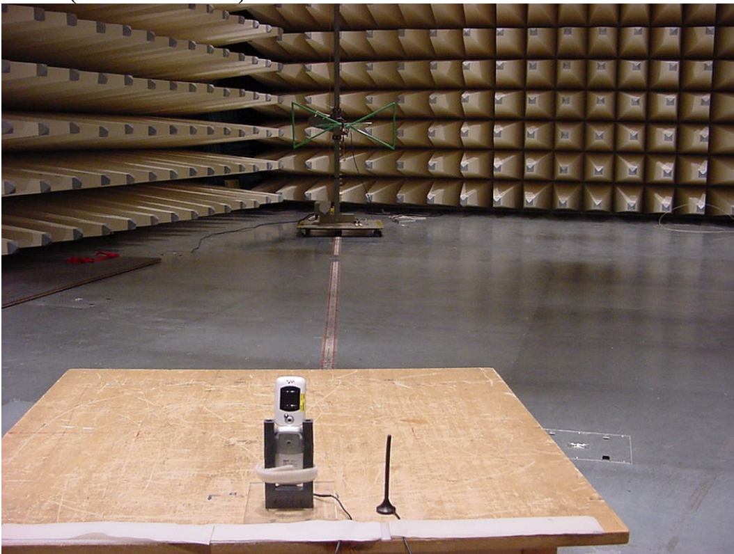
Photo 2 (Radiated Emissions):
