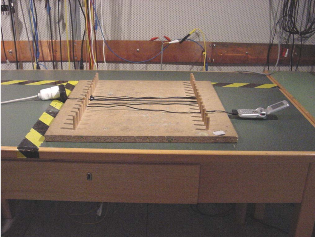
Photo 3 (Conducted Emissions):
