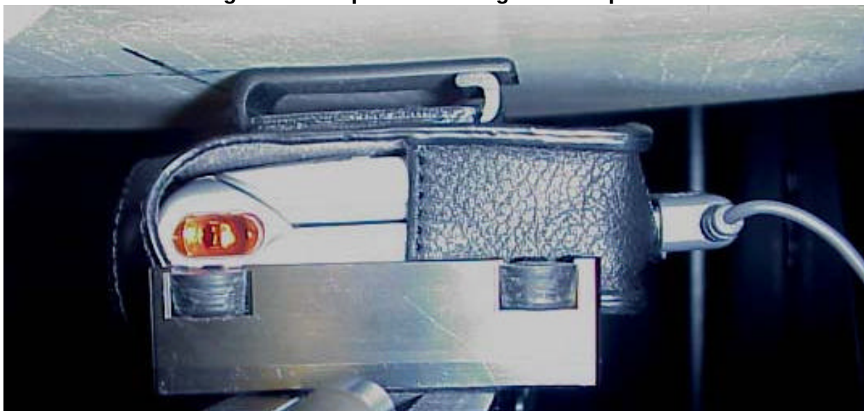
Position of device against head phantom using the “tilt” position
