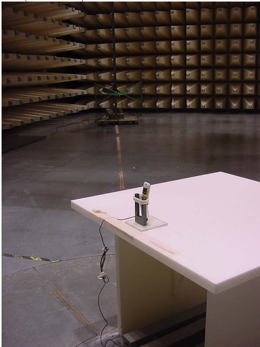
Photo 1 (Radiated Emissions):
