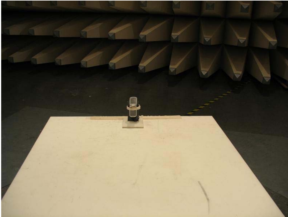
Photo 1: Radiated Emissions
