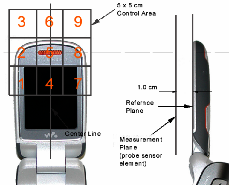
Figure 13 5x5 Scan grid above WD
