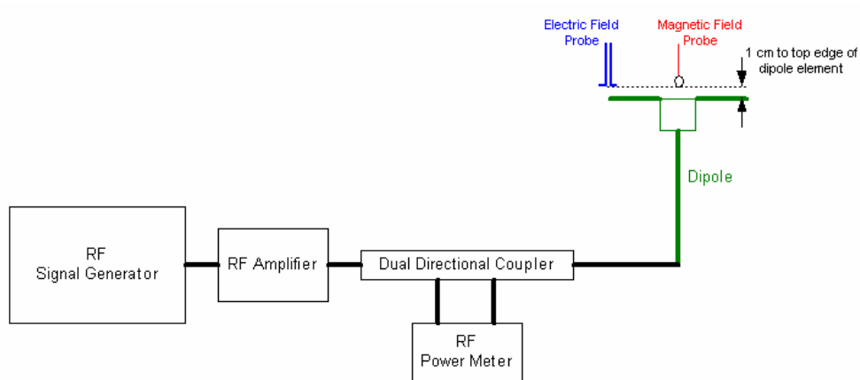
Figure 18 System Check Setup
