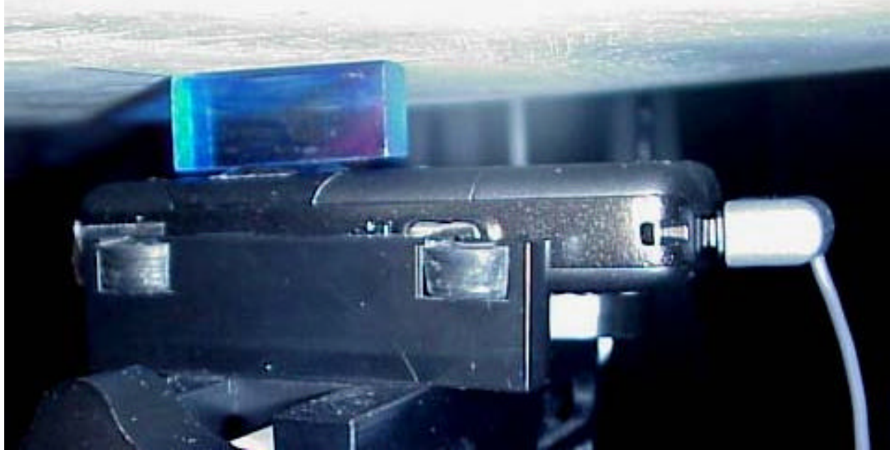
Position with back of device against flat phantom using a 15mm SPACER with hands free accessory.
