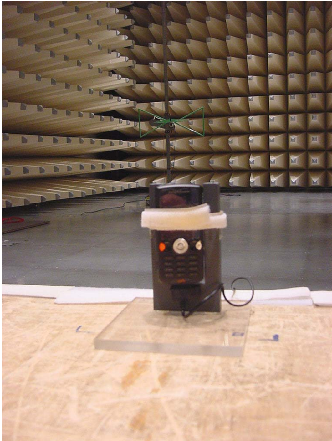
Photo 1: Radiated Emissions
