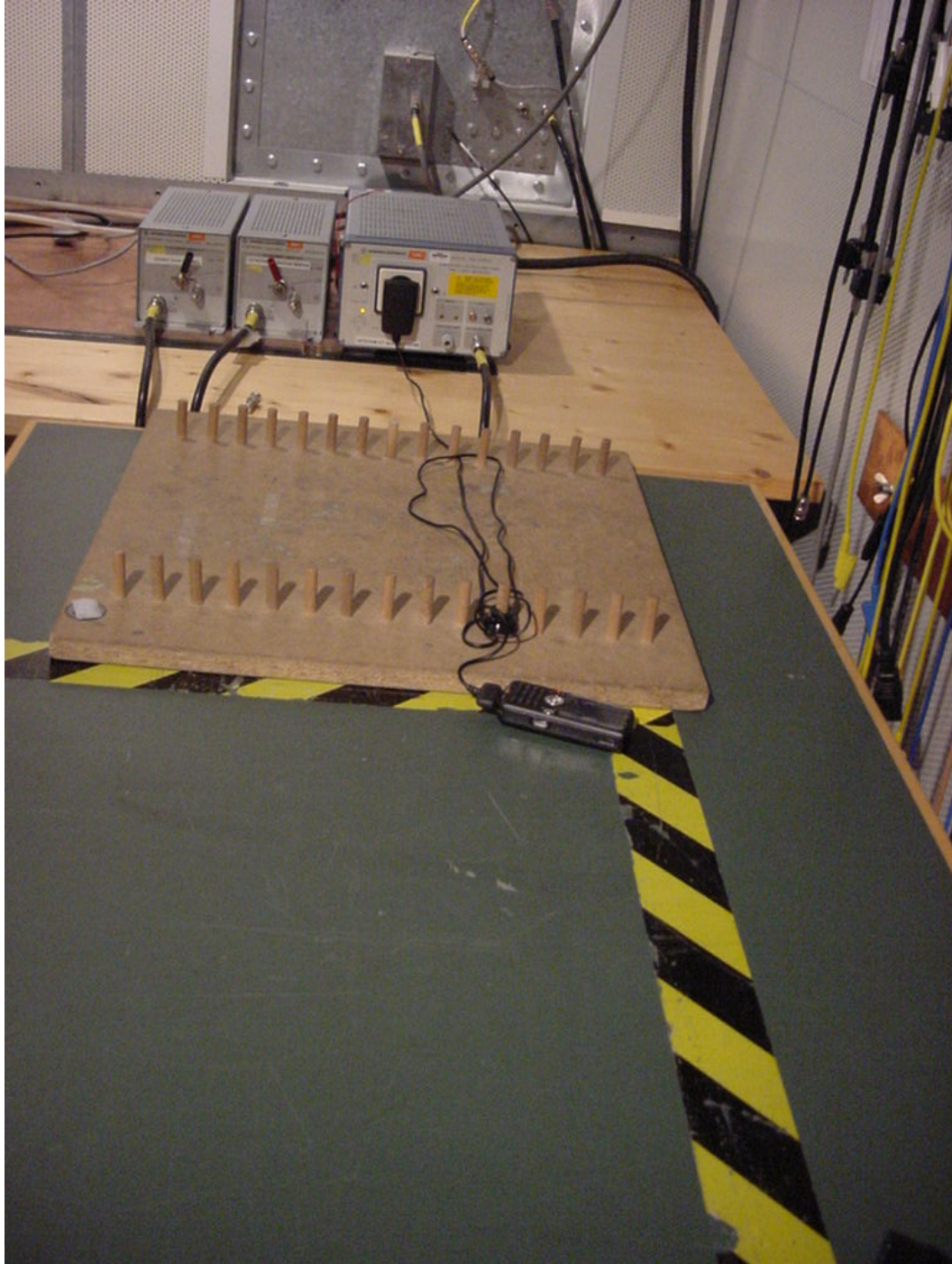
Photo 3: Conducted Emissions
