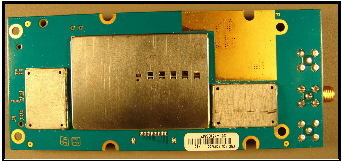
PHOTOGRAPH 5: EUT BACK VIEW
