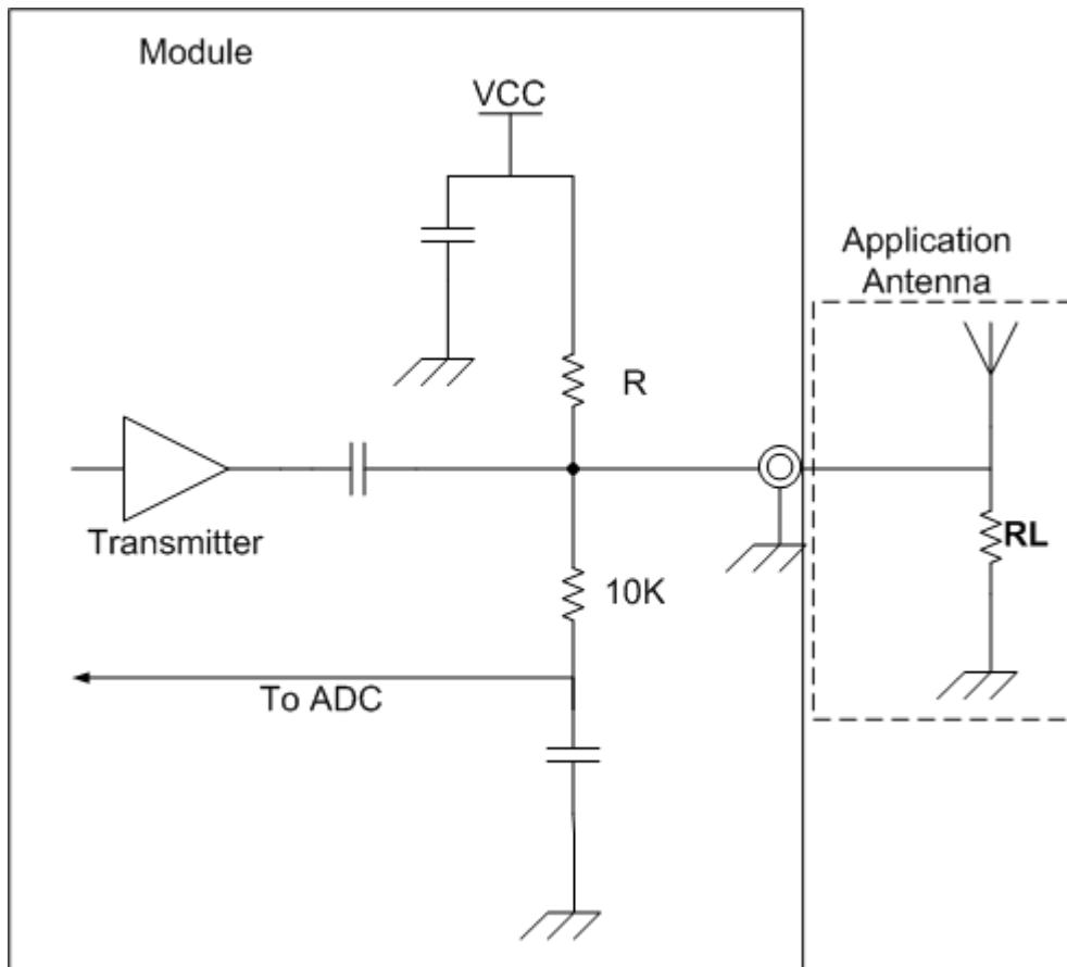
Figure 9: Antenna Diagnostic Circuit
