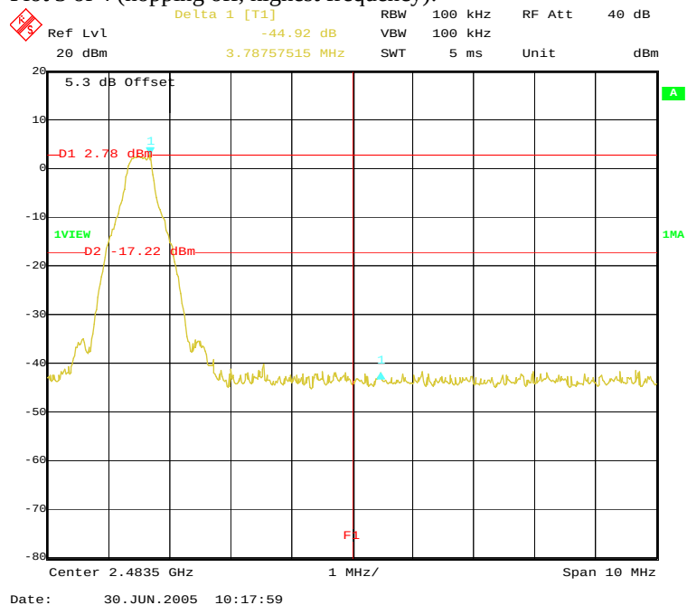
Plot 3 of 4 (hopping off, highest frequency):
