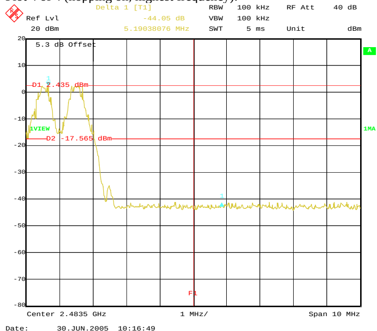
Plot 4 of 4 (hopping on, highest frequency):
