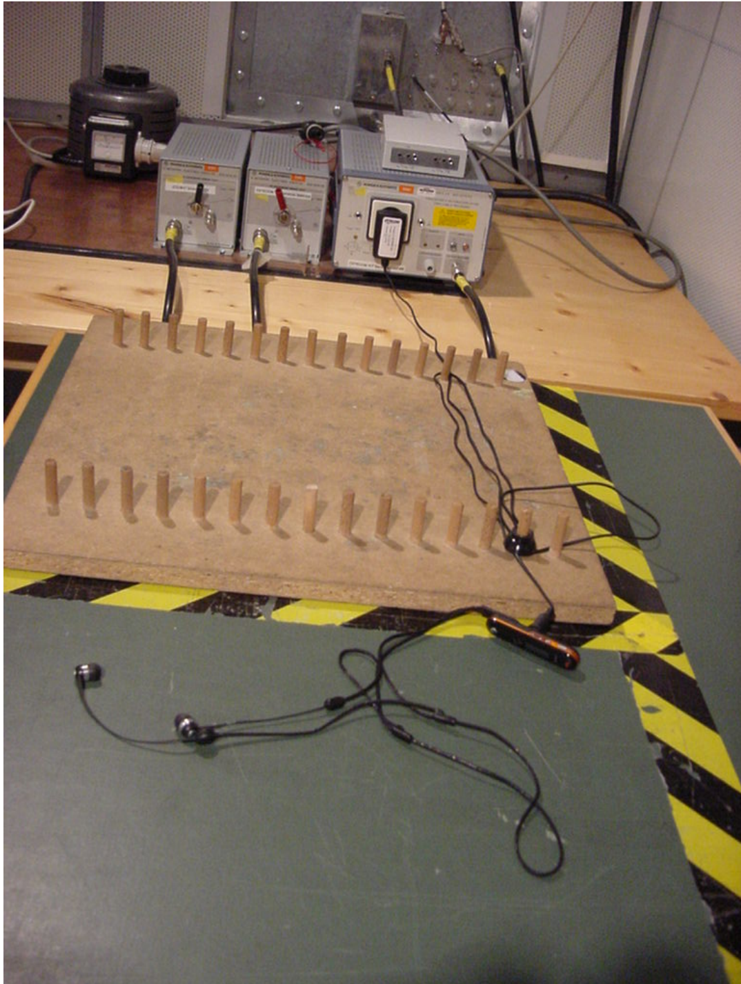
Photo 3: Conducted Emissions
