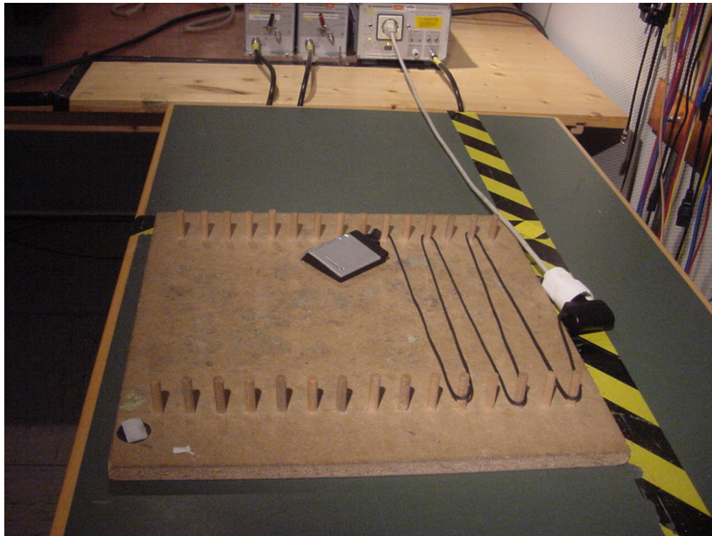
Photo 3: Conducted Emissions
