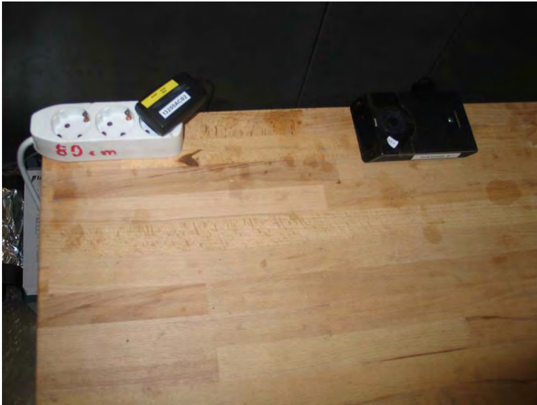
Photo 1: Test setup for conducted measurements on AC mains (setup AA_02)
