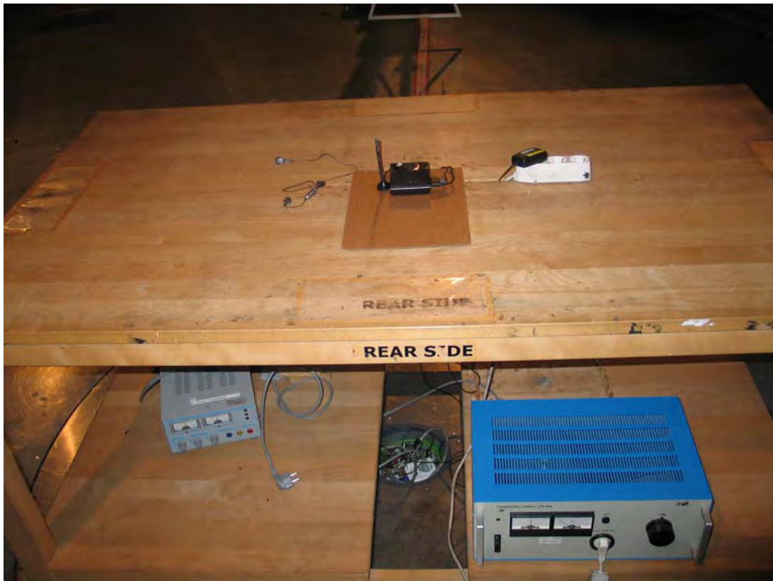
Photo 3: Test setup for radiated measurements below 1GHz (setup AC_03)
