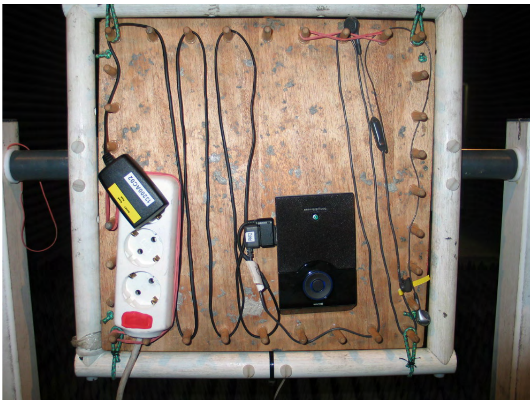
Photo 4: Test setup for radiated measurements above 1GHz (setup AC_03)
