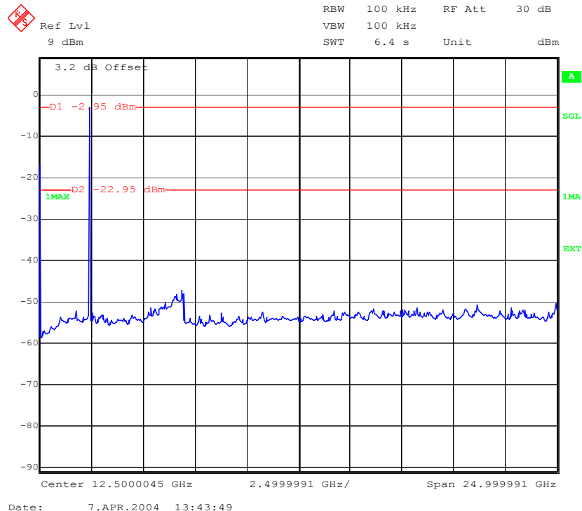
Plot 2 of 3: middle channel
