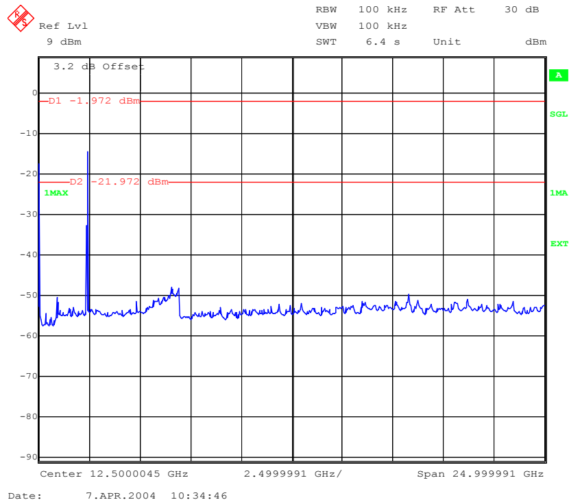
Plot 1 of 3: lowest channel
