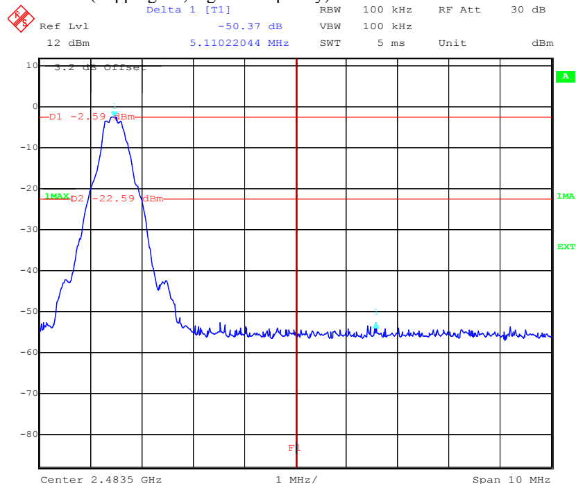
Plot 3 of 4 (hopping off, highest frequency):
