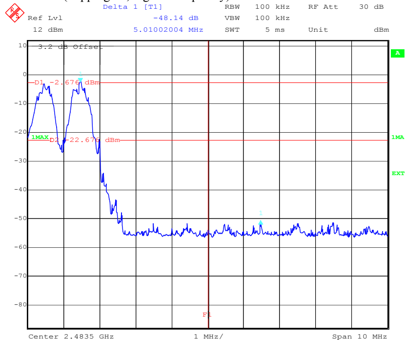
Plot 4 of 4 (hopping on, highest frequency):
