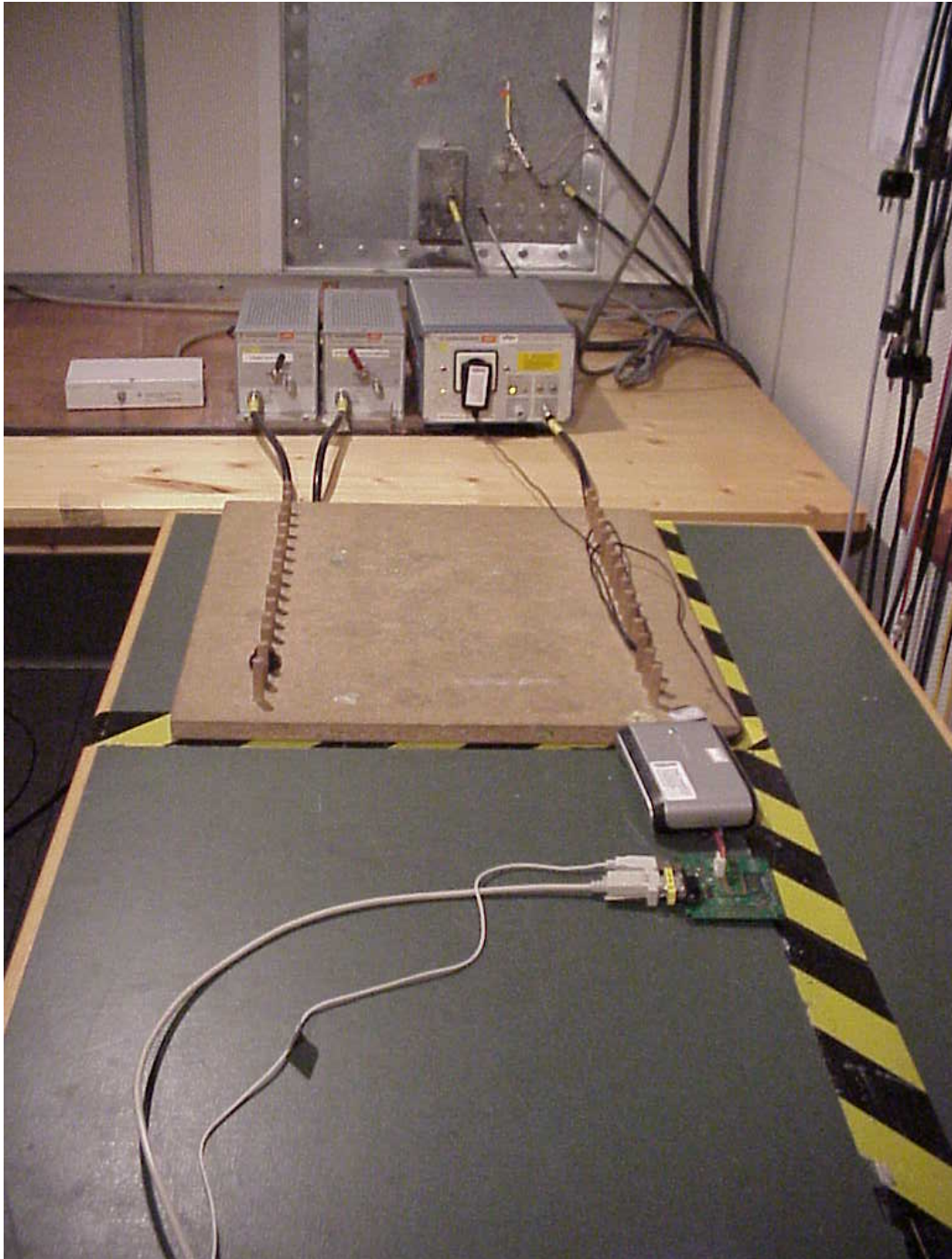
Photo 3: Conducted Emissions
