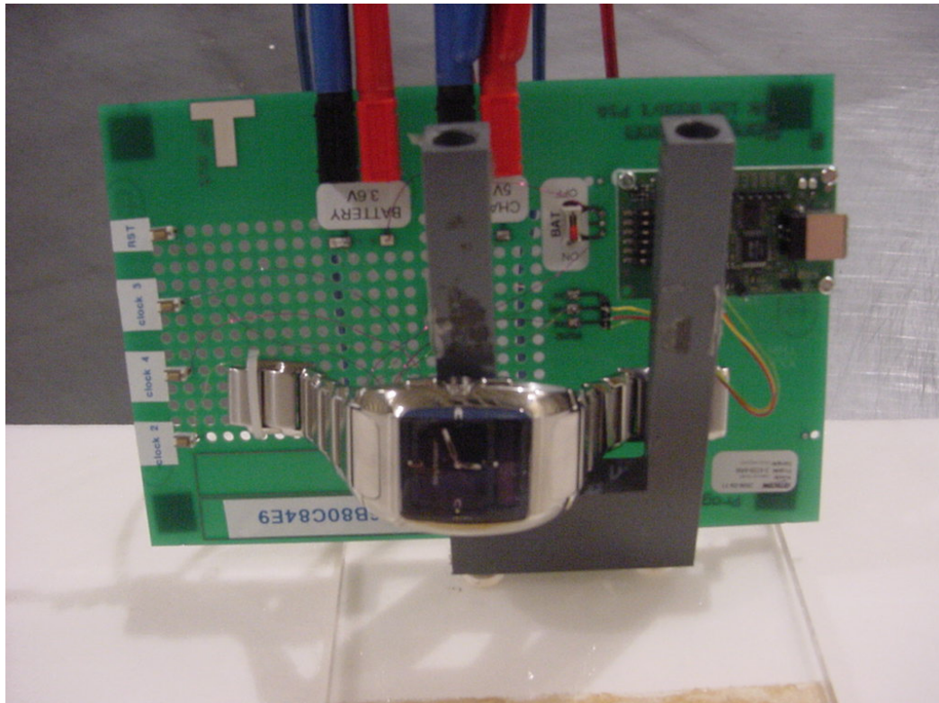
Photo 2: Radiated Emissions
