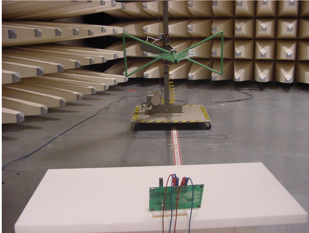
Photo 3: Radiated Emissions
