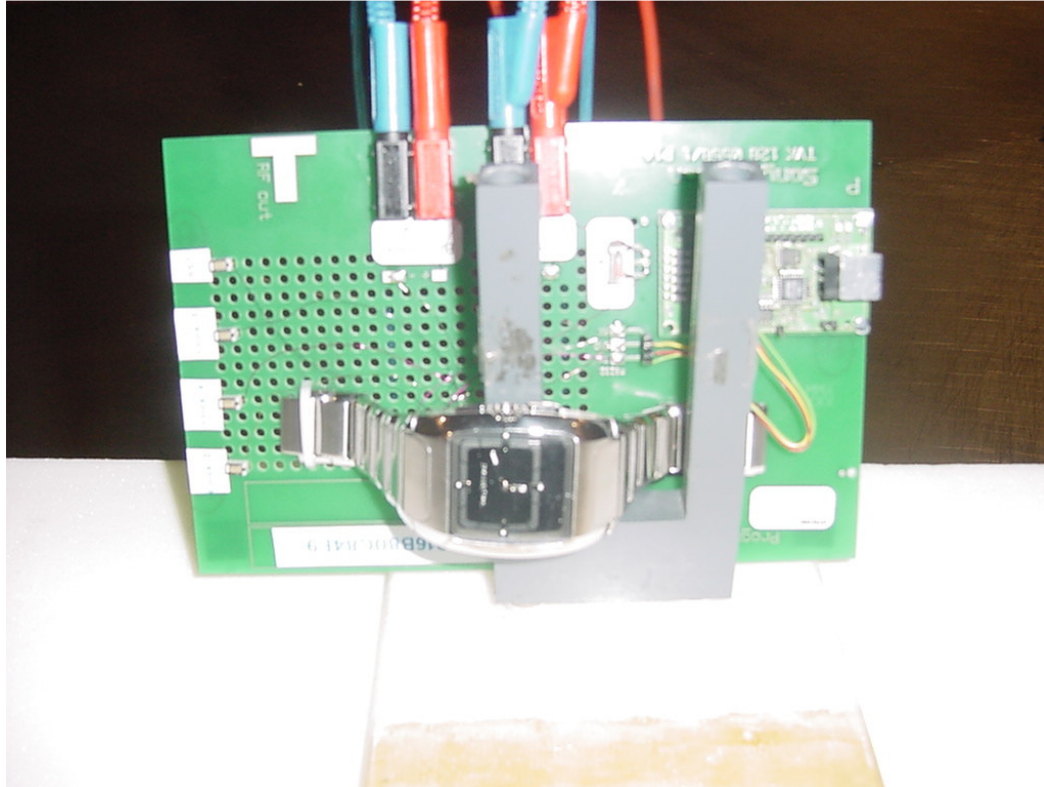
Photo 2: Radiated Emissions
