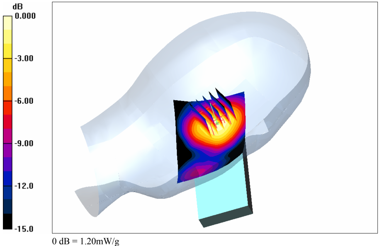
(d) Distribution of SAR in the GSM1900 mode giving the maximum 1g SAR in the left hand side phantom for the tilt position.
