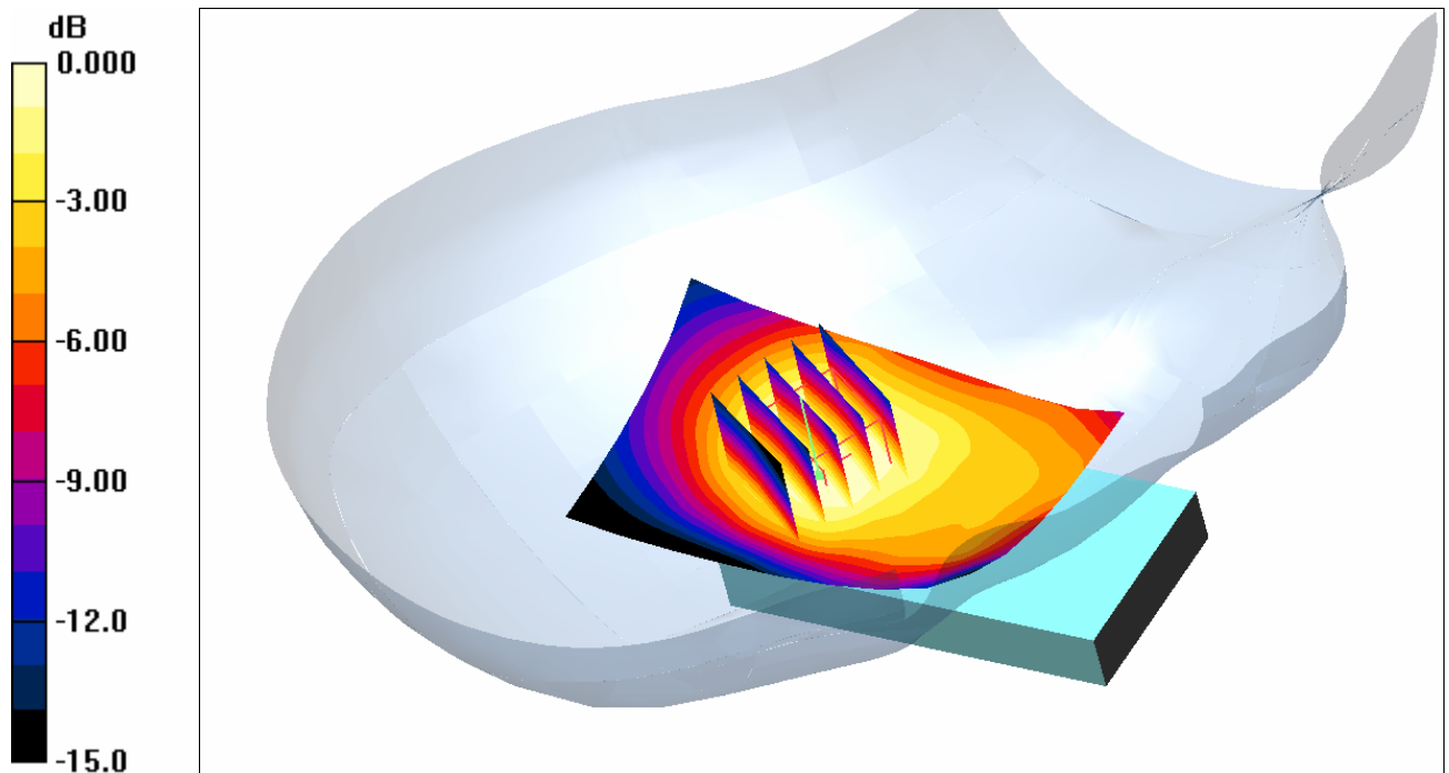
(a) Distribution of SAR in the GSM1900 mode giving the 1g SAR in the right hand side phantom for the cheek position
