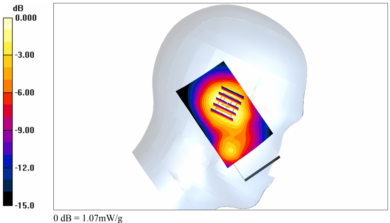
(a) Distribution of SAR in the GSM1900 mode giving the 1g SAR in the left hand side phantom for the cheek position
